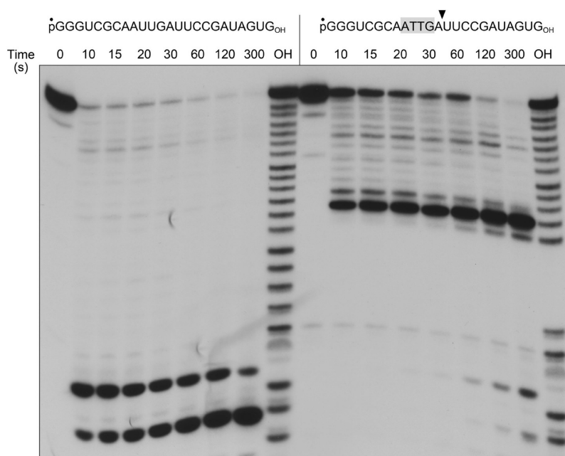
Figure 4. Tract of four internal deoxynucleotides that suffices to arrest phosphorolysis. Reaction mixtures (80 \mu L) containing 20 mM Tris-HCl (pH 7.5), 5 mM MgCl 2 , 0.5 mM (NH 4 ) 2 PO 4 , 0.3 \mu M FL PNPase protomer, and 0.1 \mu M 5'- 32 P-labeled 24-mer polynucleotide as specified, either an all-RNA strand (left) or an RNA with four consecutive internal deoxyribonucleotides (right, with deoxys highlighted in gray), were incubated at 37 °C. Aliquots (10 \mu L) were withdrawn at the specified times and reactions quenched with formamide and EDTA. The reaction products were analyzed by urea-PAGE and visualized by autoradiography. The samples in lanes OH are partial alkaline hydrolysates of the respective 5'- 32 P-labeled 24-mer polynucleotides, prepared by incubation in a solution of 40 mM NaHCO 3 and 60 mM Na 2 CO 3 (pH 10.2) for 12 min at 95 °C.
