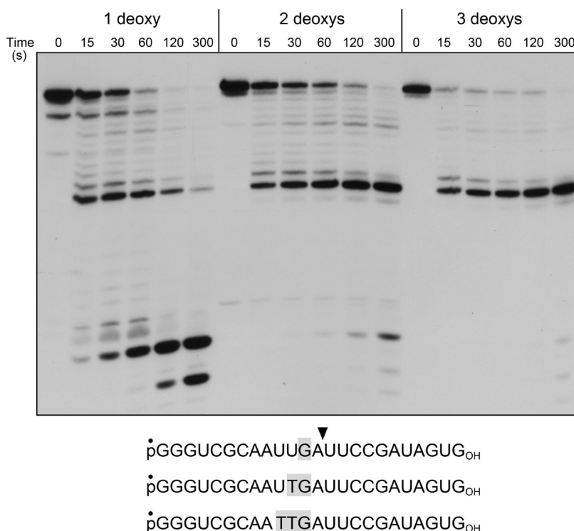
Figure 5. Effect of three internal deoxynucleotides, two internal deoxynucleotides, and one internal deoxynucleotide. Reaction mixtures (80 \mu L) containing 20 mM Tris-HCl (pH 7.5), 5 mM MgCl 2 , 0.5 mM (NH 4 ) 2 PO 4 , 0.3 \mu M FL PNPase protomer, and 0.1 \mu M 5'- 32 P-labeled 24-mer RNA with three internal deoxynucleotides, two internal deoxynucleotides, or one internal deoxyribonucleotide (shown at bottom, with deoxys highlighted in gray) were incubated at 37 °C. Aliquots (10 \mu L) were withdrawn at the specified times and reactions quenched with formamide and EDTA. The reaction products were analyzed by urea-PAGE and visualized by autoradiography.
