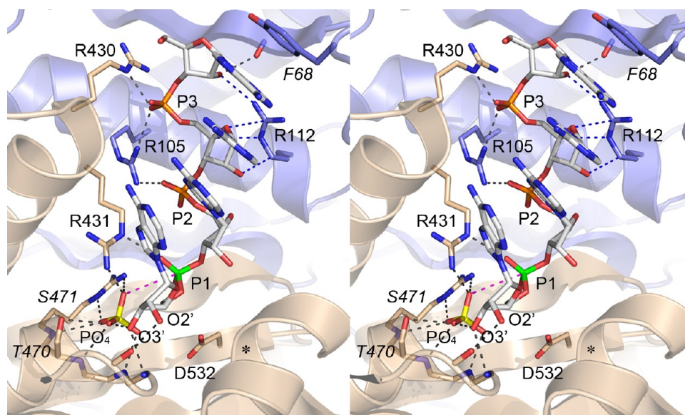
Figure 8. Insights into PNPase catalysis from the archaeal exosome structure. Stereoview of the active site of the archaeal exosome (from PDB entry 4BA2) with an RNA OH and inorganic phosphate bound. The polypeptides corresponding to the proximal and distal PH domains in PNPase are colored blue and beige, respectively. The phosphorus atom of the 3'-terminal phosphodiester is colored green. The path of nucleophilic attack of the phosphate anion (depicted with a yellow phosphorus atom) on the scissile phosphodiester (P1) is denoted by the magenta dashed line. Hydrogen bonding and electrostatic contacts with the RNA and inorganic phosphate ligands are denoted by dashed black lines. The side chains are labeled and numbered according to their counterparts in mycobacterial PNPase. Identical side chains are labeled in regular font. Nonidentical side chains are labeled in italic font.
