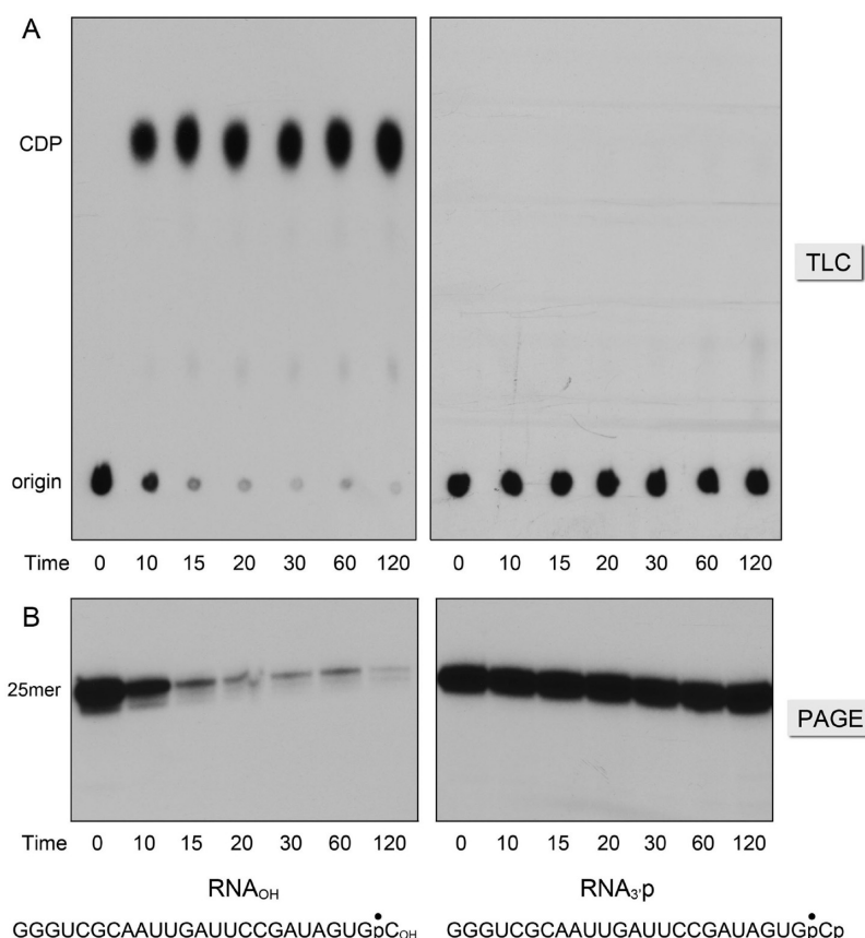
Figure 6. Can PNPase process dirty 3'-PO 4 ends? Phosphorolysis of 3'- 32 P-labeled 25-mer RNA p or RNA OH substrates (shown at the bottom) by full-length PNPase in the presence of magnesium was assayed as described in Experimental Procedures. The reactions were quenched at the specified times (s) and the products analyzed in parallel by PEI-cellulose TLC (A) and urea-PAGE (B).
