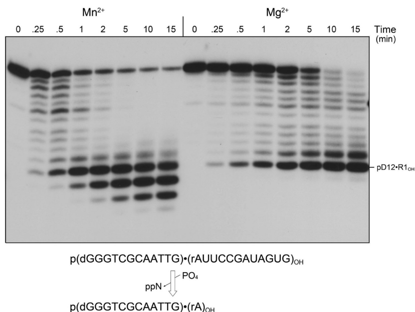
Figure 3. Time course of pDNA•RNA OH phosphorolysis. Reaction mixtures (80 \mu L) containing 20 mM Tris-HCl (pH 7.5), 5 mM MnCl 2 or 5 mM MgCl 2 as specified, 30 \mu M (NH 4 ) 2 PO 4 , 0.1 \mu M 5'- 32 P-labeled pDNA•RNA OH substrate, and 0.3 \mu M ΔS1 PNPase protomer were incubated at 37 °C. Aliquots (10 \mu L) were withdrawn at the specified times and reactions quenched with formamide and EDTA. The reaction products were analyzed by urea-PAGE and visualized by autoradiography.
