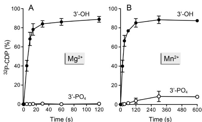
Figure 7. Kinetics of processing of 3'-OH vs 3'-PO 4 substrates. Phosphorolysis of 3'- 32 P-labeled 25-mer RNap or RNA OH substrates by full-length PNPase in the presence of magnesium (A) or manganese (B) was assayed as described in Experimental Procedures. The reactions were quenched at the specified times and the products analyzed by PEI-cellulose TLC. The extent of [ 32 P]CDP release (as a percentage of total radioactivity) is plotted as a function of reaction time. Each datum in the graphs is the average of three separate experiments ± the standard error of the mean.
