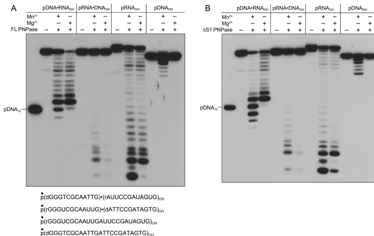
Figure 2. DNA imposes a kinetic obstacle to 3'-phosphorolysis. Reaction mixtures (10 \mu L) containing 20 mM Tris-HCl (pH 7.5), 5 mM MnCl 2 or 5 mM MgCl 2 (where indicated by +), 30 \mu M (NH 4 ) 2 PO 4 , 0.1 \mu M 5'- 32 P-labeled 24-mer polynucleotide substrate as specified (either pDNA OH , pRNA OH , or pDNA•RNA OH or pRNA•DNA OH chimeras, shown at the bottom with the radiolabel denoted by ●), and either 0.1 \mu M full-length PNPase protomer (A) or 0.3 \mu M ΔS1 PNPase protomer (B) were incubated for 15 min at 37 °C. The products were resolved by urea-PAGE and visualized by autoradiography. A 5'- 32 P-labeled 12-mer DNA strand, pGGGTCGCAATTG OH (pDNA 12 ), corresponding to the DNA segment of the pDNA•RNA chimera was analyzed in parallel in the left lanes of the gels.
