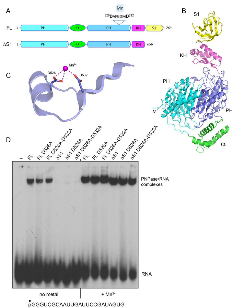
Figure 1. Domain organization of mycobacterial PNPase and effects of metal ligand mutations on nucleic acid binding. (A) Modular domain structures of full-length (FL) M. smegmatis PNPase and the \Delta S1 variant. The sequence motif comprising the metal-binding site in the distal PH domain is highlighted. (B) Tertiary structure of the homologous FL PNPase of Caulobacter crescentus [Protein Data Bank (PDB) entry 4AIM]. (C) Mn^{2+} -binding site in the Escherichia coli PNPase- Mn^{2+} crystal structure (PDB entry 3GME). The aspartates are numbered according to their position in M. smegmatis PNPase. (D) Electrophoretic mobility-shift assay of RNA binding by FL and \Delta S1 PNPase performed as described in Experimental Procedures. The free ^{32}P -labeled 24-mer RNA (sequence shown at bottom) and slower-migrating PNPase- [^{32}P] nucleic acid complexes were resolved by native polyacrylamide gel electrophoresis and visualized by autoradiography.
